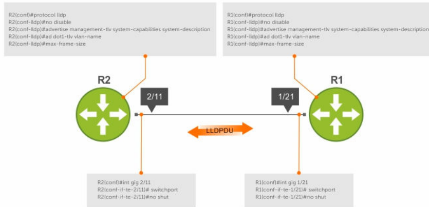
Figure 72. Configuring LLDP
